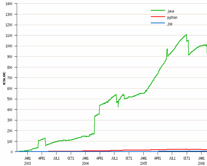
Figure 2 – SirsiDynix lines of new Java code in thousands from 2003-2006.
